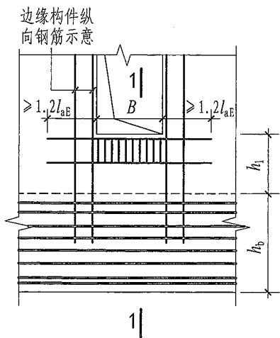
( B \leq 2h_1 且 h_1 \geq h_b/2 )
