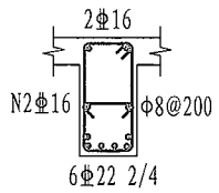
2-2 300 × 550
