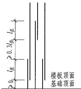
(a) 绑扎搭接
