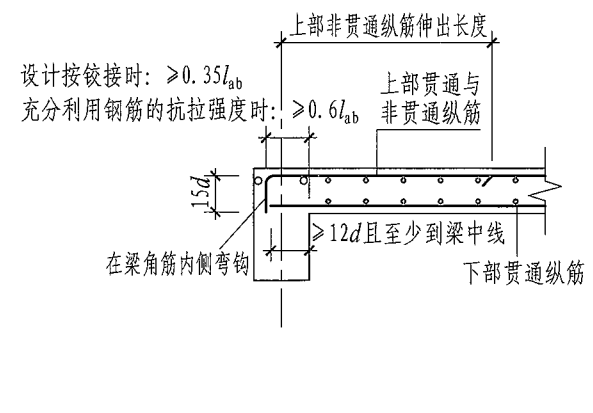
(c) 跨中板带与梁连接
