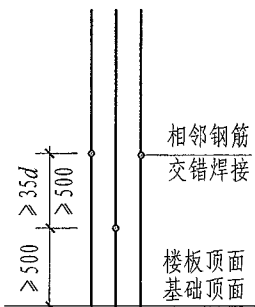
(c) 焊接
