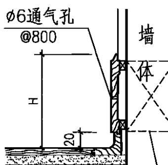
(a) 防腐木砖 60X120X120
